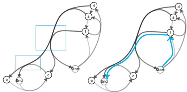
Fig. 15. Rectangles indicate regions causing the curve from d to e to be more visually salient. Thus, when looking for a path from start to end, the blue path may be less likely to be found than the path via d.
